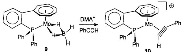
Scheme 3. \text{DMA}^+ = dimethylanilinium ( \text{PhNMe}_2 \text{H}^+ )
