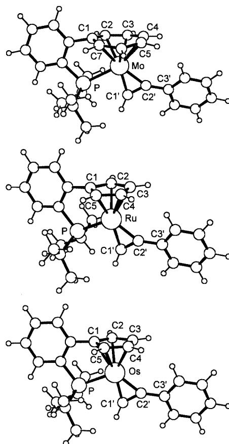
Figure 5. Calculated structures of the cations 7 , 11 , and 12
