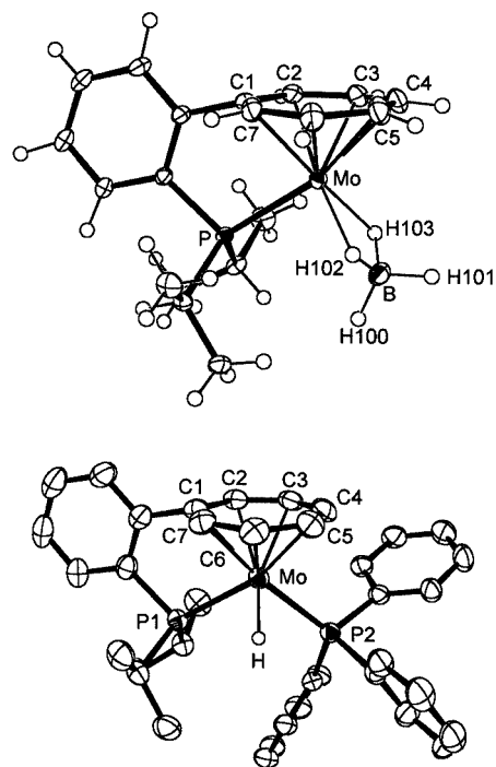
Figure 1. ORTEP drawings of 3 (top) and 4 (bottom) with thermal ellipsoids drawn at 50% probability
