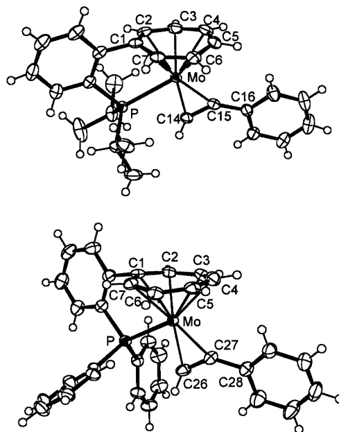
Figure 4. ORTEP drawings of the cations in (7)BPh 4 (top) and (10)BPh 4 ·C 6 H 14 (bottom) with thermal ellipsoids drawn at 50% probability
