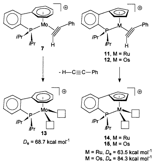
Scheme 5. Alkyne bond dissociation energies ( D_e ) of phenylacetylene complexes
