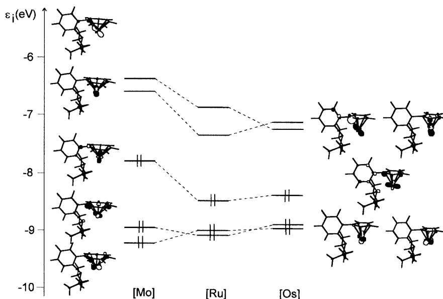
Figure 6. Frontier orbitals of the 14-electron complexes 13 [M = Mo], 14 [M = Ru], and 15 [M = Os]
