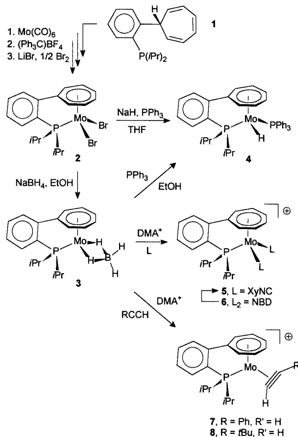
Scheme 2. XyNC = 2,6-dimethylphenyl isocyanide; NBD = 2,5-norbornadiene; \text{DMA}^+ = \text{dimethylanilinium} (\text{PhNMe}_2 \text{H})^+
