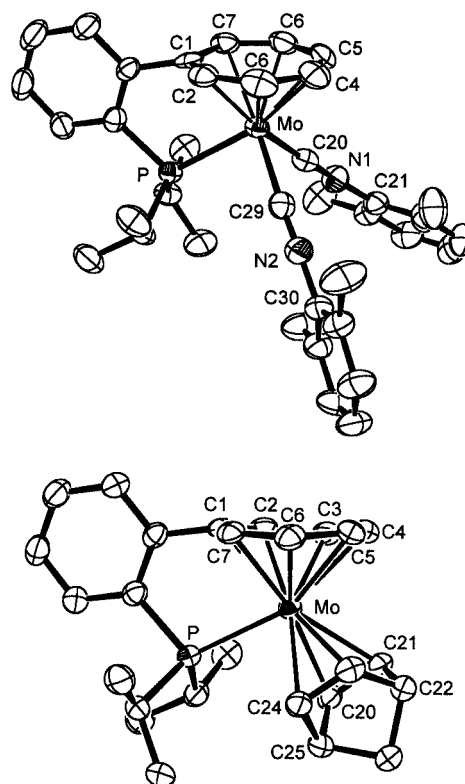
Figure 3. ORTEP drawings of the cations in ( 5 ) \text{BPh}_4\cdot\text{C}_5\text{H}_{12} (top) and ( 6 ) \text{BPh}_4\cdot\text{CH}_2\text{Cl}_2 (bottom) with thermal ellipsoids drawn at 50% probability
