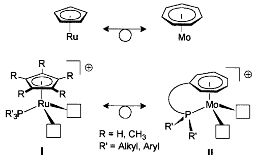
Scheme 1. Isolobal relationship between cyclopentadienyl ruthenium and cycloheptatrienyl molybdenum complex fragments
