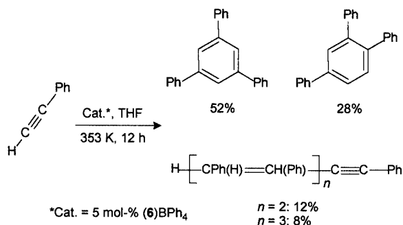
Scheme 4. Catalytic oligomerization of phenylacetylene
