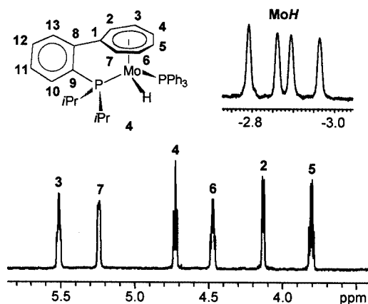
Figure 2. Selected parts of the ^1\text{H} NMR spectrum (600 MHz, [\text{D}_8]\text{toluene} ) of 4
